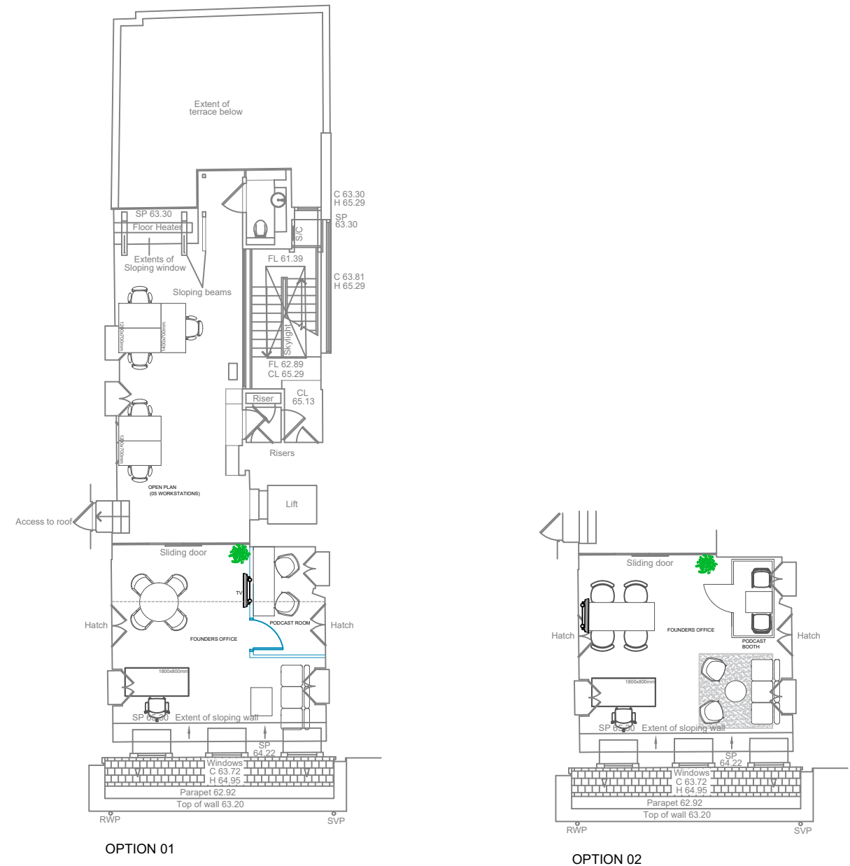
FOURTH FLOOR
